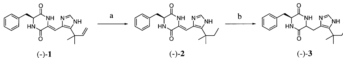
Scheme 1. (a) H 2 /10% Pd-C, MeOH, rt, 2 h; (b) H 2 /10% Pd-C, MeOH, rt, 24 h.
