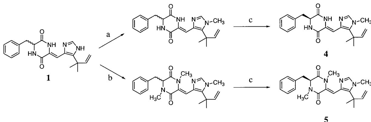
Scheme 2. (a) MeI, NaH, DMF, -30°C, 2 h; (b) MeI, NaH, DMF, rt, 2 h; (c) chiral HPLC.
