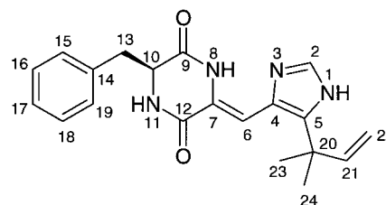
Figure 1. Structure of (-)-phenylahistin [(-)-1].
