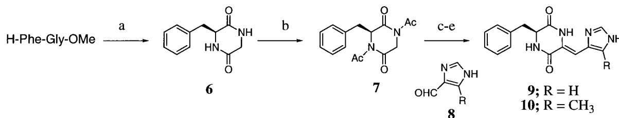
Scheme 3. (a) MeOH, reflux, 14 h; (b) Ac 2 O, AcONa, 80°C, 14 h; (c) 8 LDA, HMPA, DMF, -60°C, 0.5 h; (d) Tf 2 O, pyridine, rt, 10 min; (e) NH 4 OH, rt, overnight.
